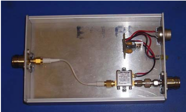
Fig. 3: Left: opened frontend with preamplifier. Right: Noise figure measured with a Callisto.
