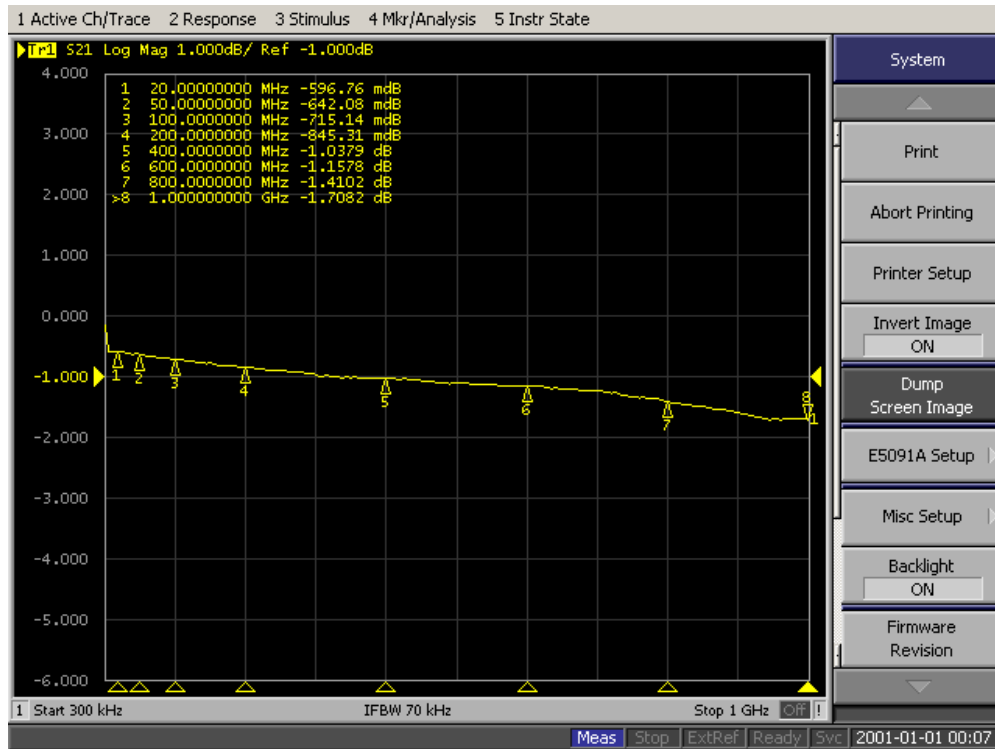
Fig. 3: Measurement of s_{21} between antenna port and LNA-port with < 2dB up to 1 GHz. For low loss application such as in L-band rf-microwave relays are required. This is not part of this project as cost will be much higher with rf-microwave relays. Plot of Calu-24-01
